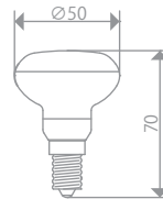
LDF002-SM
