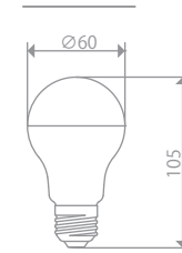
LDF80D, LDF81D
