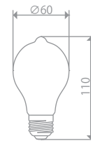
LDF29D, LDF44D
