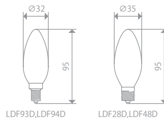
LDF93D, LDF94D
