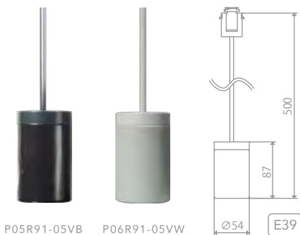
P05R91-05VB P06R91-05VW
