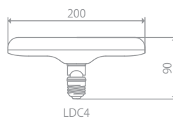
LDC4
