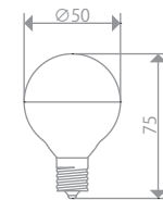
LDF92D, LDF71D
