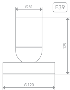
SLB1
